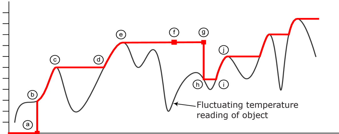
Fig. 7-2 Graphical representation of typical Peak temperature measurement
